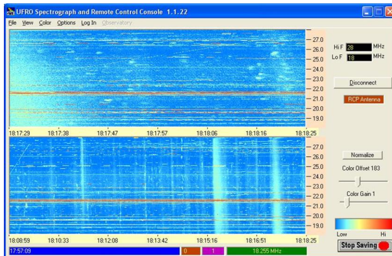
Figure 10. This is an example display of some solar bursts using the Spectrograph software. The upper panel is a 1-minute window and the lower panel is a 10-minute window (Credit: Jim Sky).
