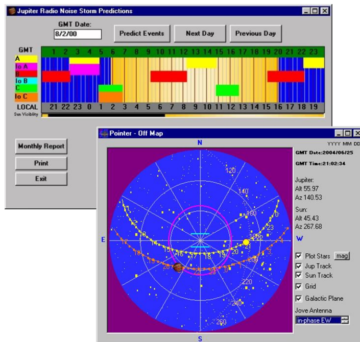
Figure 9. A screenshot of the Radio Jupiter Pro software program for planning Jupiter and solar observations (Credit: Jim Sky).
